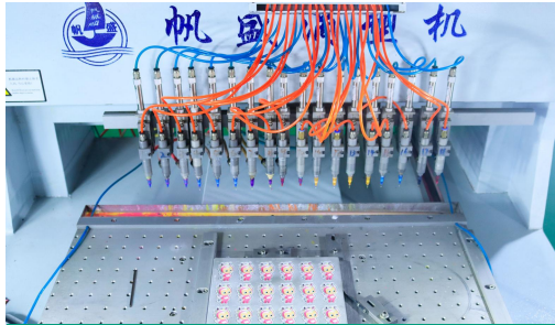
Dispensing Equipment
