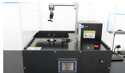
Flip-top Testing Machine
